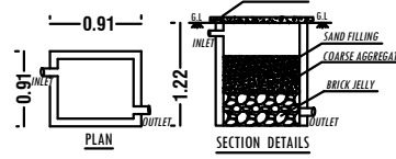
RAINWATER HARVESTING SYSTEM
