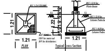
FOOTING DETAILS
