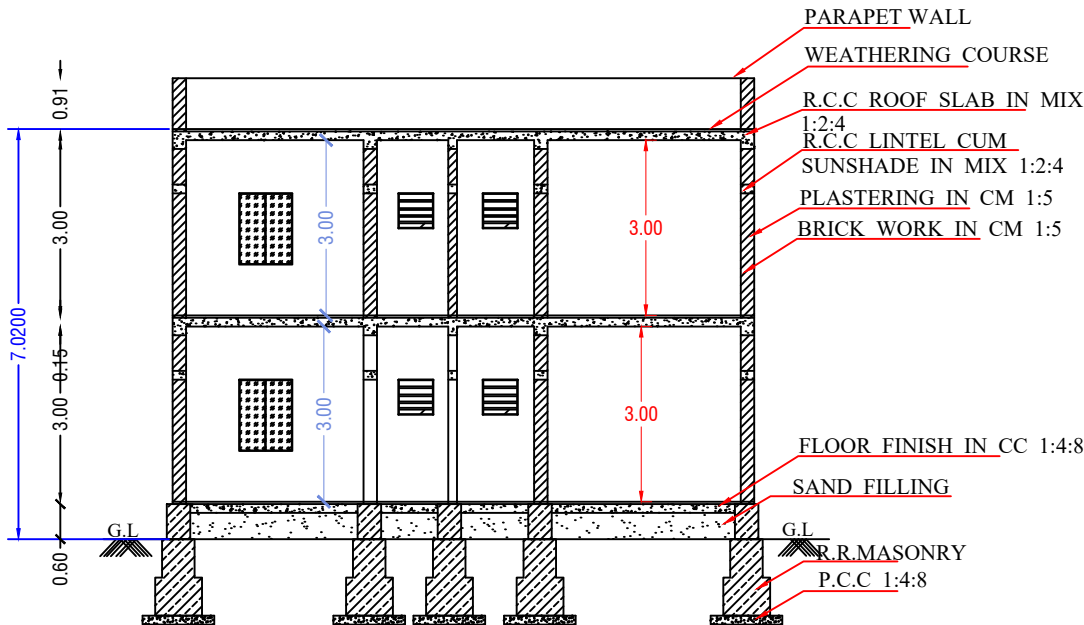
SECTION ON-"AB"
