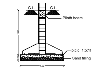
FOUNDATION DETAILS
