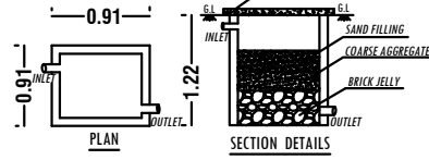
RAINWATER HARVESTING SYSTEM
