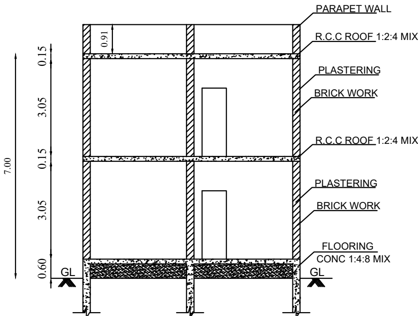
SECTION 'US'
