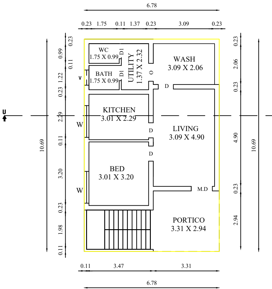
Extg.GROUND FLOOR PLAN
