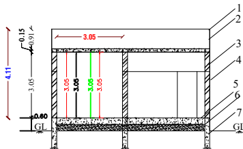
SECTION ON 'MS'
