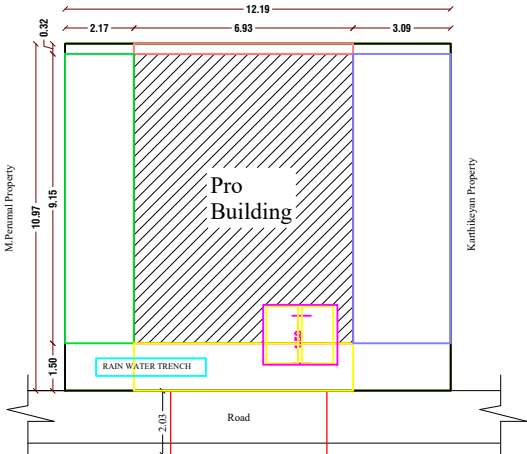
Sit Plan SCALE 1:100
