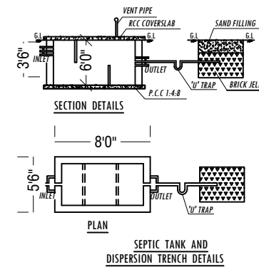
SEPTIC TANK AND DISPERSION TRENCH DETAILS
