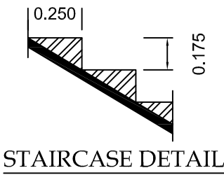
STAIRCASE DETAIL
