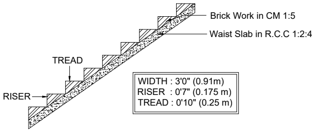
STAIRCASE DETAILS
