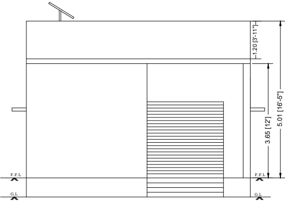
FRONT ELEVATION
