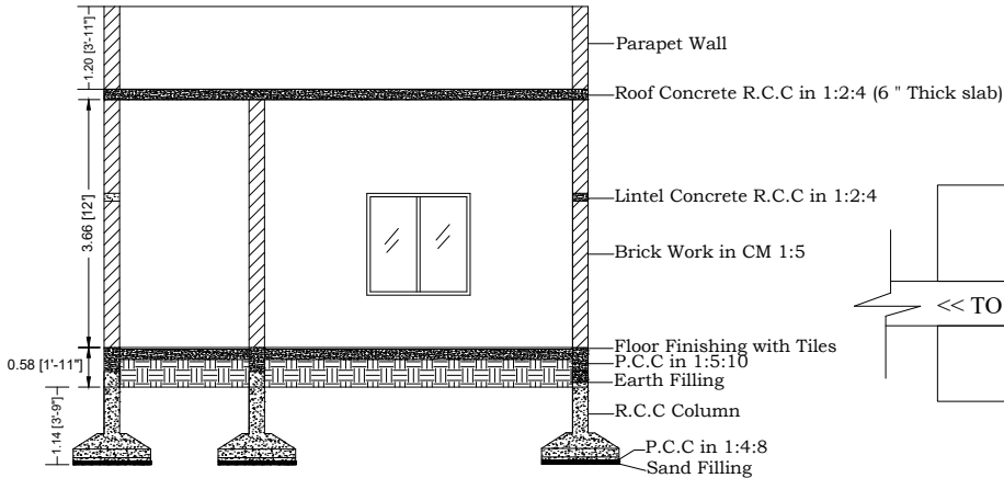
SECTION X-X
