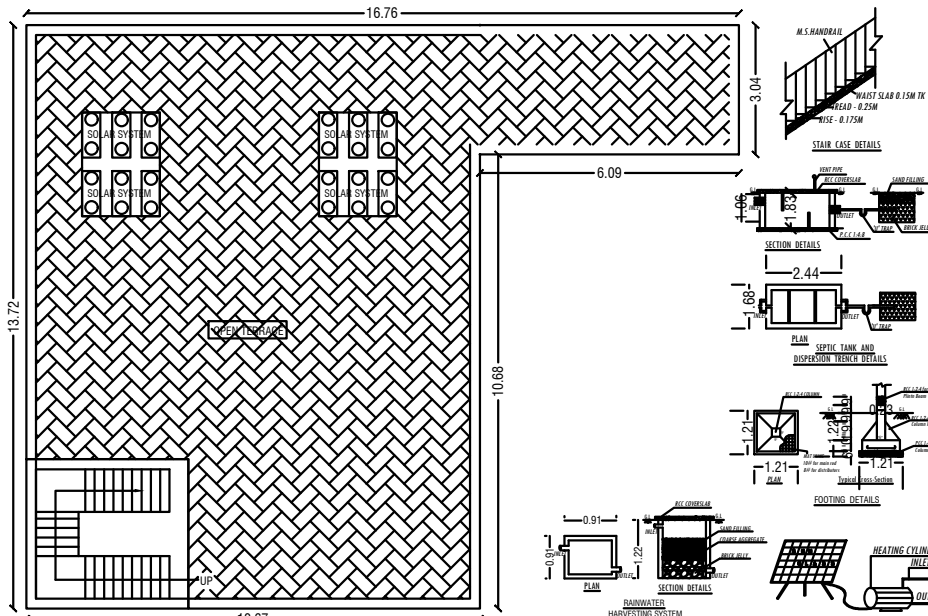
OPEN TERRACE FLOOR PLAN
