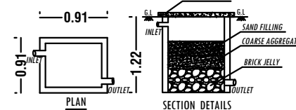
RAINWATER HARVESTING SYSTEM
