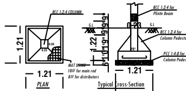
FOOTING DETAILS
