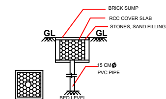
RAIN WATER HARVESTING TANK (NOT TO SCALE)
