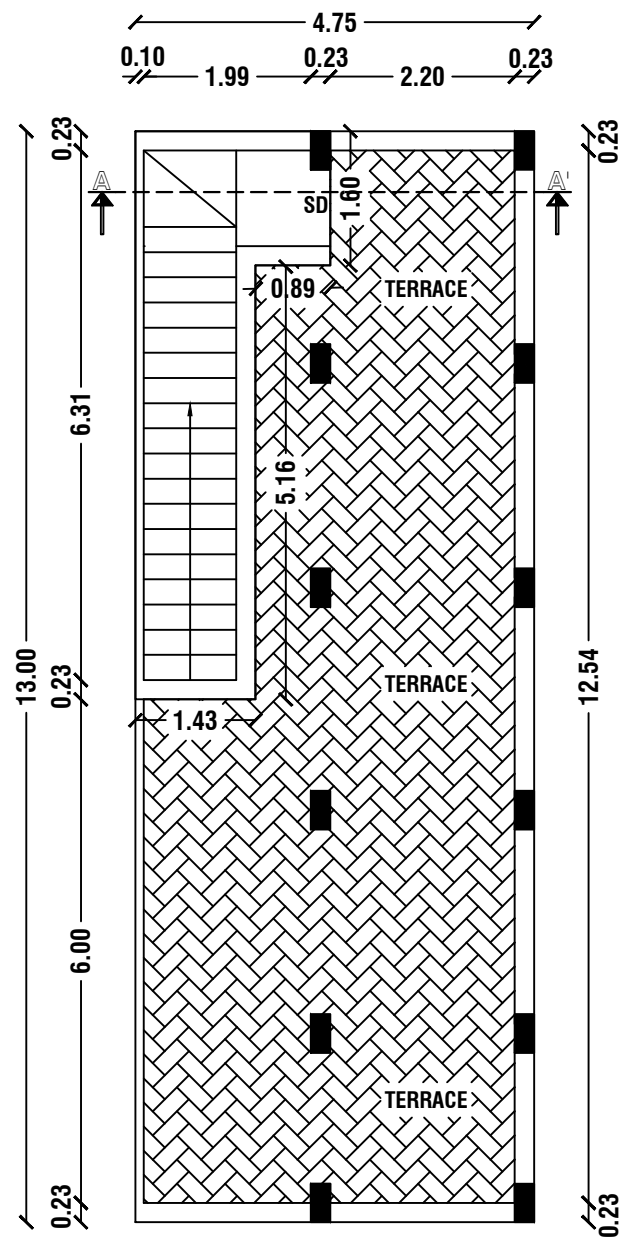
OPEN TERRACE FLOOR PLAN
