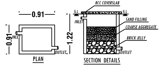
RAINWATER HARVESTING SYSTEM
