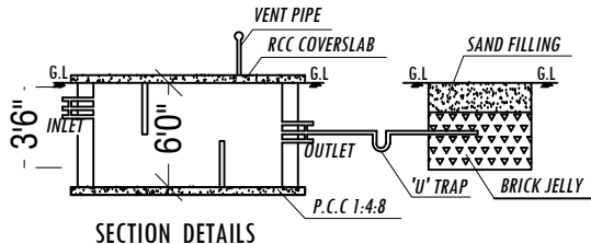
SECTION DETAILS
