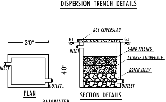
SEPTIC TANK AND DISPERSION TRENCH DETAILS
