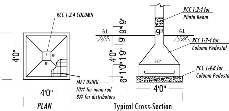
FOOTING DETAILS
