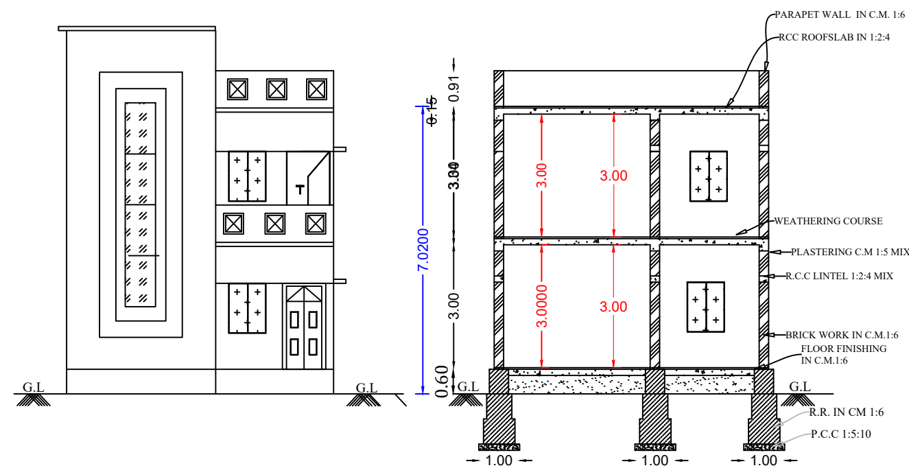
FRONT ELEVATION
