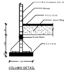
COLUMN DETAIL
