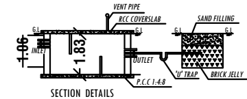
SECTION DETAILS
