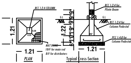
FOOTING DETAILS
