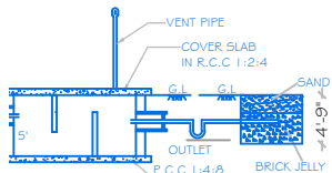
SECTION-AB
