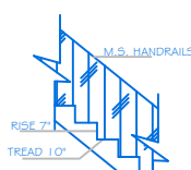
STAIRCASE DETAILS
