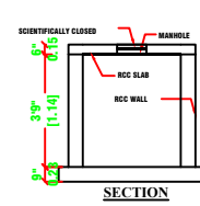
SUMP DETAILS
