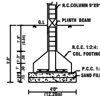
FOUNDATION DETAILS
