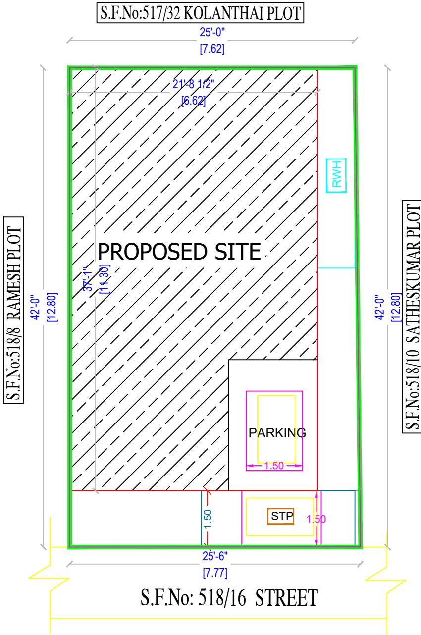
SITE PLAN
