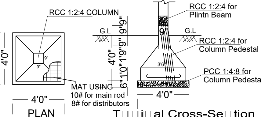
FOOTING DETAILS
