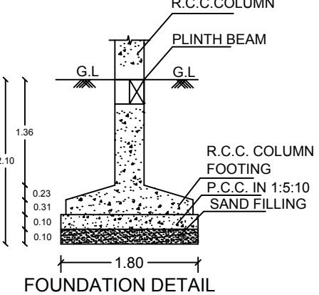
FOUNDATION DETAIL (DETAILS C)
