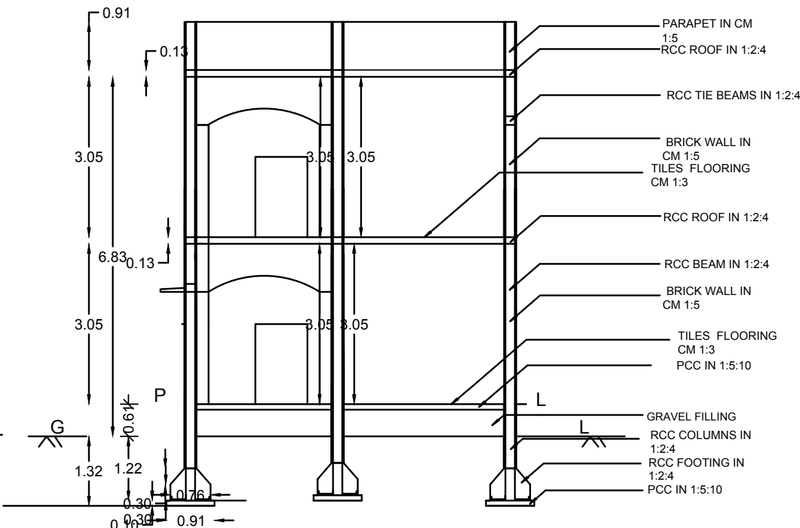
SECTION :A-A'
