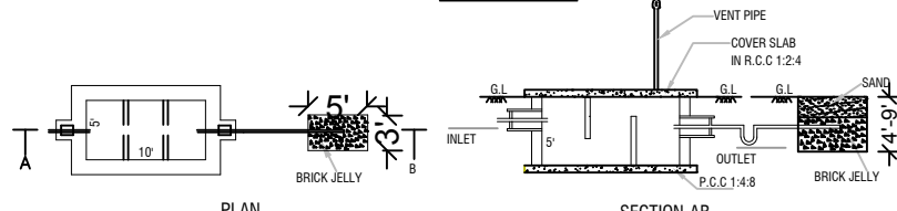
SECTION-AB
