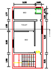
PROPOSED SECOND FLOOR PLAN
