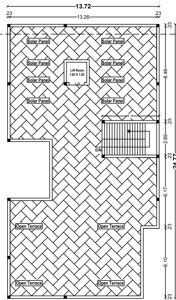
Terrace Floor
