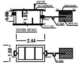
PLAN SEPTIC TANK AND DISPERSION TRENCH DETAILS
