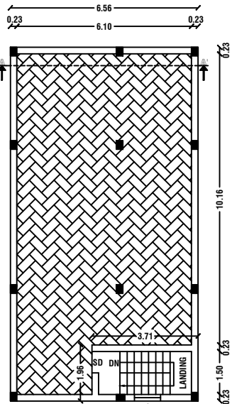
OPEN TERRACE FLOOR PLAN
