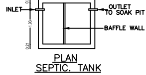
SECTION OF SEP.TANK
