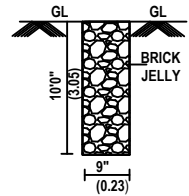
PERCULATION PIT
