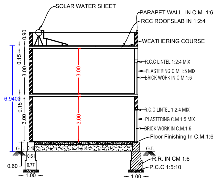
SECTION ON-'AB'
