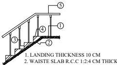
1. LANDING THICKNESS 10 CM 2. WAISTE SLAB R.C.C 1:2:4 CM THICK 3. RISE 15 CM 4. TREAD 25CM 5. HANDRAIL HEIGHT 80 CM Staircase Details
