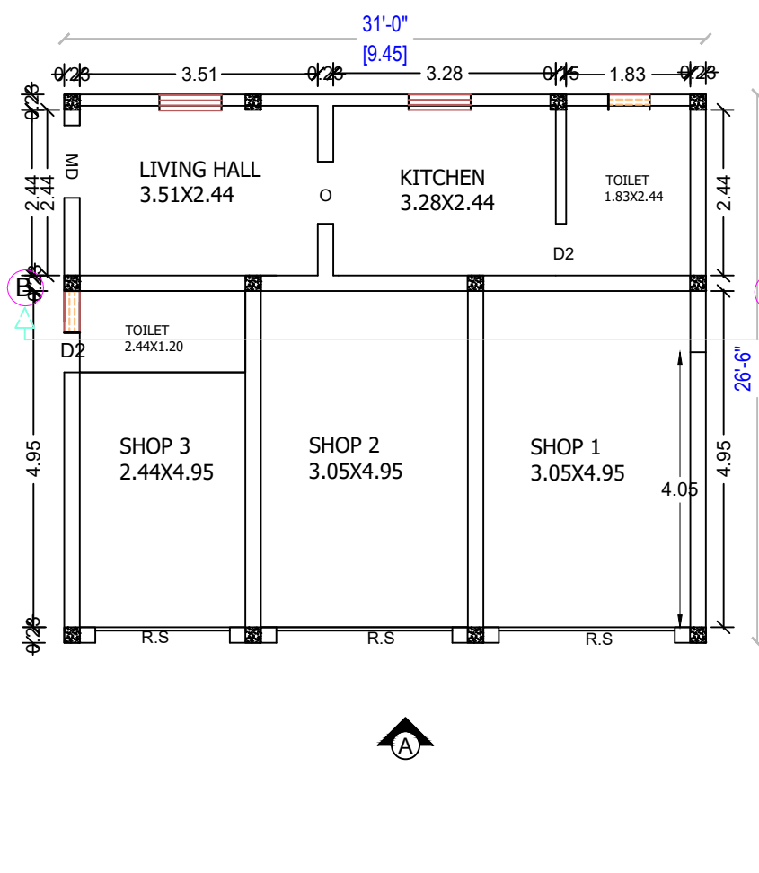
GROUND FLOOR ALTERATION PLAN
