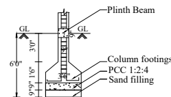
FOUNDATION DETAILS SCALE 1:50
