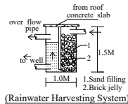
(Rainwater Harvesting System)
