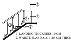
Staircase Details
