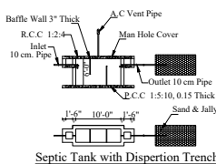
Septic Tank with Dispersion Trench
