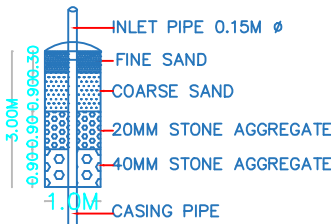
DETAILS OF RAIN WATER HARVESTING STRUCTURES
