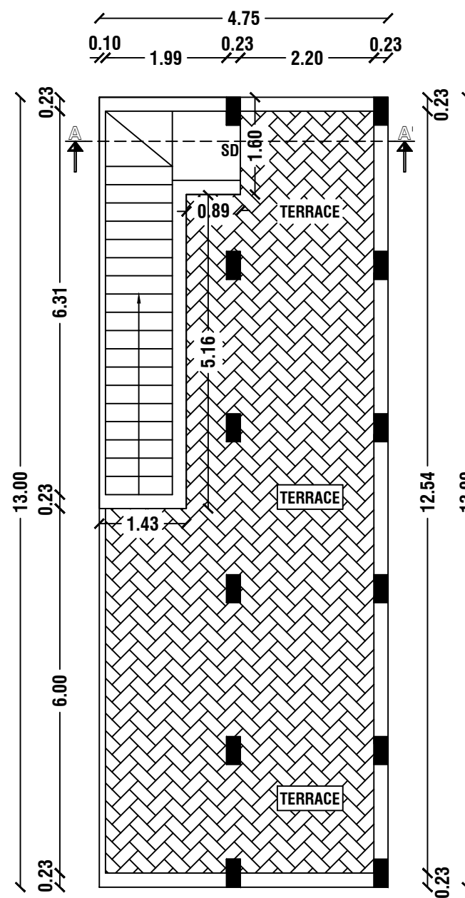
OPEN TERRACE FLOOR PLAN
