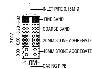
DETAILS OF RAIN WATER HARVESTING STRUCTURES
