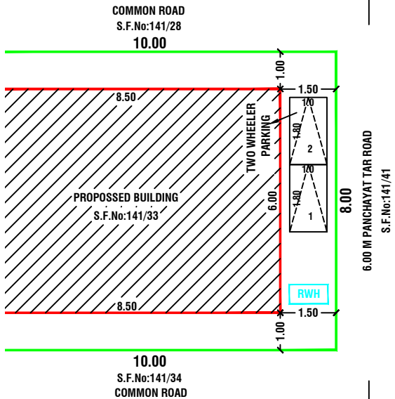
SITE PLAN SCALE 1:100 & As Per FMB AND VAO BOUNDARY CERTIFICATE
