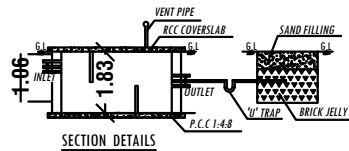
SECTION DETAILS
