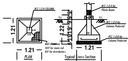
FOOTING DETAILS
