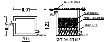
RAINWATER HARVESTING SYSTEM
