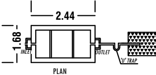
PLAN SEPTIC TANK AND DISPERSION TRENCH DETAILS
