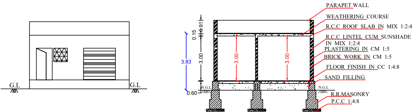
FRONT ELEVATION
