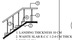
Staircase Details
