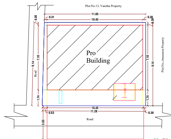
Sit Plan SCALE 1:100
