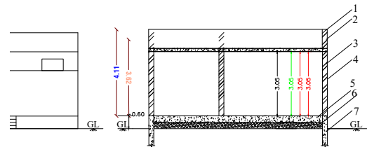
SECTION ON 'KV'
