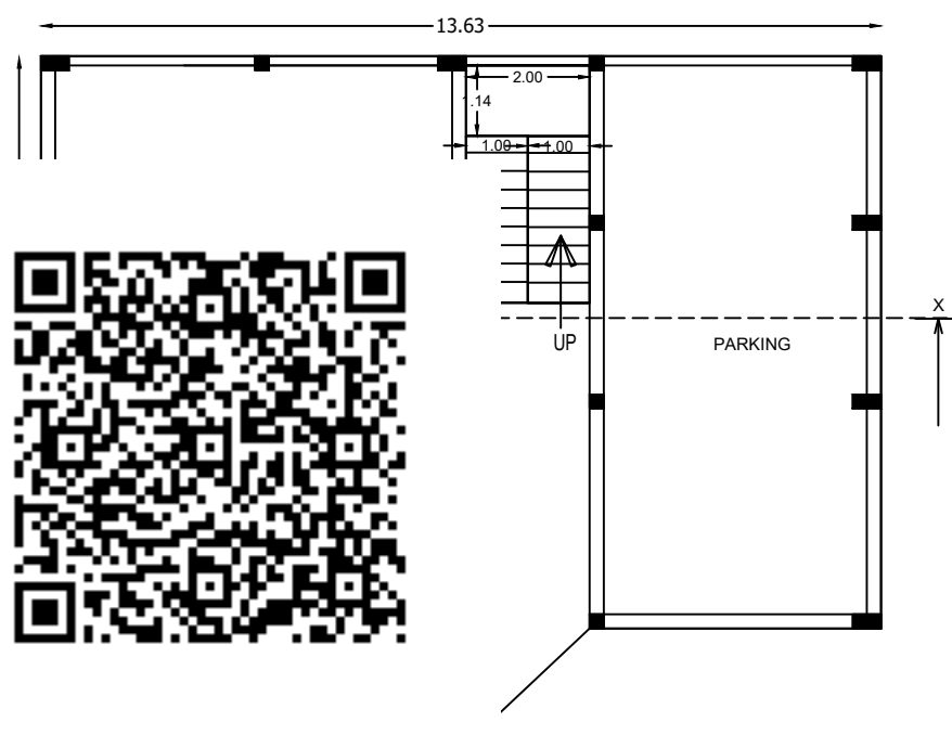
STILT FLOOR
