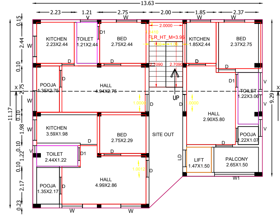
SECOND FLOOR
