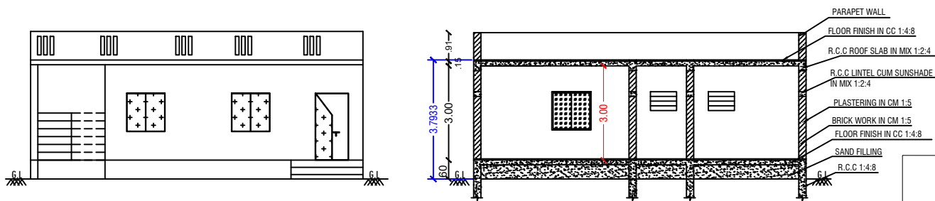
ELEVATION PLAN
