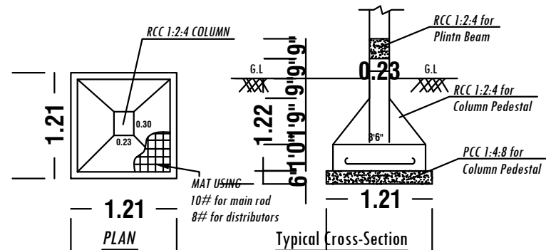
FOOTING DETAILS
