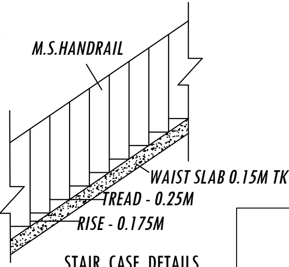
STAIR CASE DETAILS
