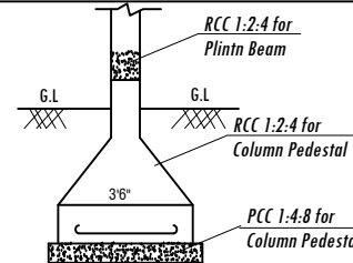
Typical Cross-Section
