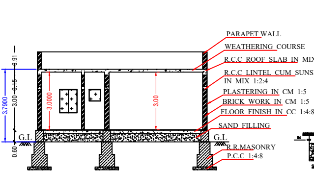
SECTION ON-'AB'
