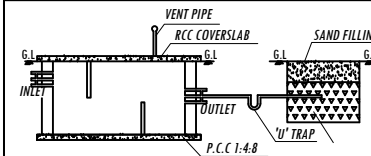
SECTION DETAILS
