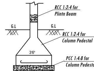
Typical Cross-Section FOOTING DETAILS
