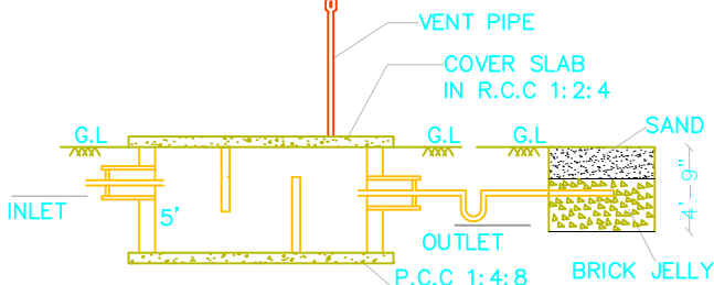
SECTION-AB
