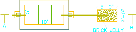
SEPTIC TANK & DISPERSION TRENCH DETAILS SCALE- 1:100
