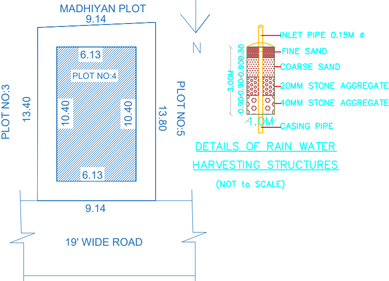
SITE PLAN
