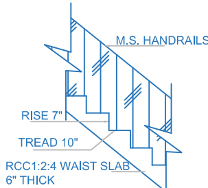
STAIRCASE DETAILS SCALE- 1:20
