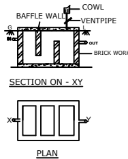
SEPTICTANK DETAILS
