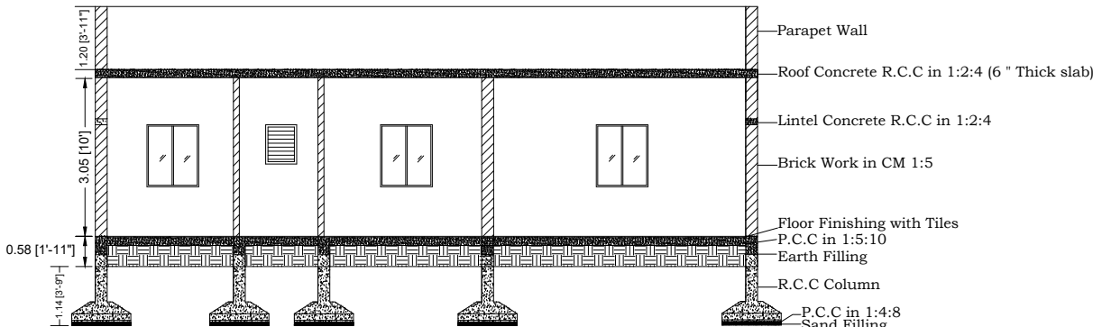
SECTION X-X
