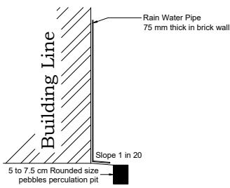
RAINWATER HARVESTING
