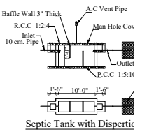
Septic Tank with Disperser
