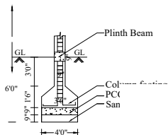
FOUNDATION DETAIL SCALE 1:50
