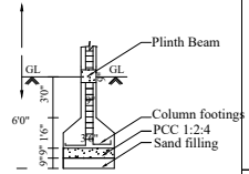
Foundation Details (Scale 1:50)
