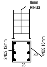
COLUMN DETAILS (NOT TO SCALE)
