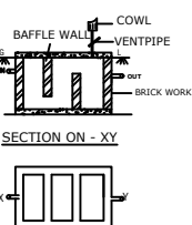
SEPTICTANK DETAILS NOT TO SCALE
