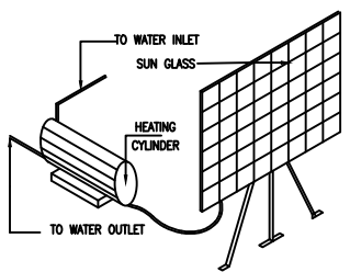
SOLAR WATER HEATING SYSTEM SCALE : N.T.S.
