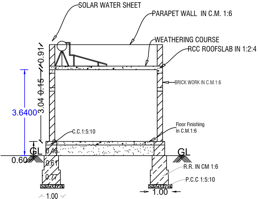
SECTION ON-"AB
