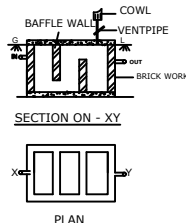
SEPTICTANK DETAILS NOT TO SCALE
