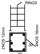
COLUMN DETAILS (NOT TO SCALE)
