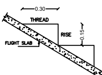
STAIRCASE DETAILS (NOT TO SCALE)
