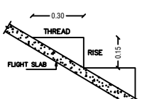
STAIRCASE DETAILS (NOT TO SCALE)
