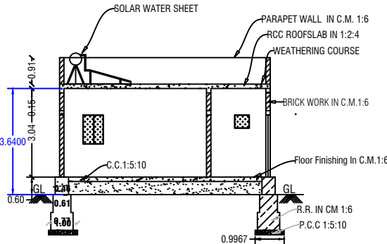
SECTION ON-'AB'
