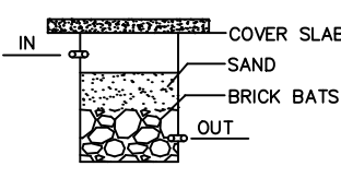
RAINWATER HARVEST NOT TO SCALE
