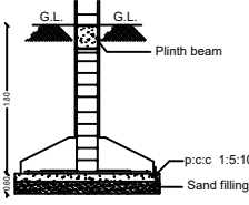
FOUNDATION DETAILS
